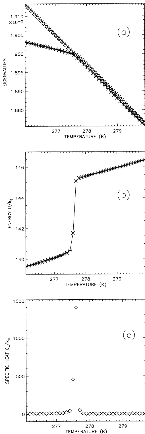
FIG. 6. (a) The three lowest eigenvalues of the transfer integral operator. The asterisk corresponds to \varepsilon_0 , the diamond to \varepsilon_1 , and the triangle to \varepsilon_2 . (b) The evolution of the energy versus T . (c) The evolution of the specific heat on the same interval of temperature. The parameters are \alpha = 0.35 , D = 0.03 eV, a = 4.5 \text{ \AA}^{-1} , K = 0.06 eV/ \text{\AA} , \rho = 1.0 , and m = 300 amu.
