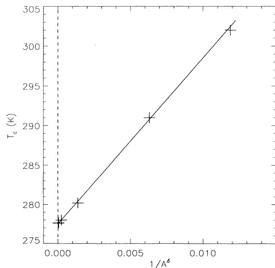
FIG. 3. Value of the critical temperature (defined by the peak of the specific heat) versus 1/A^\delta , where A is the upper bound of the integral. The five different points correspond to A = 195, 95, 45, 20, 10 , and 7.5 . The fitting parameter \delta is 2. The parameters are \alpha = 0.35 , D = 0.03 \text{ eV} , a = 4.5 \text{ \AA}^{-1} , K = 0.06 \text{ eV/\AA} , \rho = 1.0 , and m = 300 \text{ amu} .
